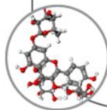
Flavonol glycosides
